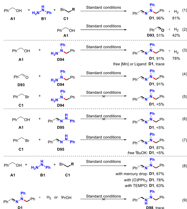
Fig. 2 Mechanistic investigations.
