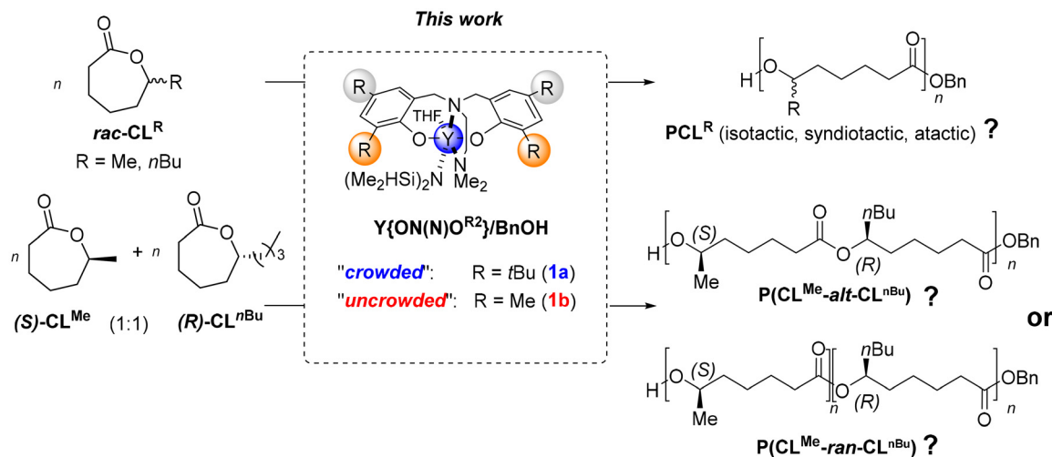
Scheme 3 ROP of 1-substituted- \epsilon -caprolactones ( rac\text{-CL}^R ; R = \text{Me}, n\text{Bu} ) and ROCOP of equimolar mixtures of opposite-configuration, enantiopure monomers studied in the present work to assess the stereoselectivity ability of discrete yttrium complexes towards such seven-membered lactones.
