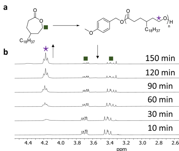
Fig. 1 (a) ROP of \gamma\text{C}_{18}\text{CL} using DPP (10 mol%), 4-methoxybenzyl alcohol ( [\text{M}]_0/[\text{I}]_0 = 50 ), benzene- d_6 . (b) Stacked ^1\text{H} NMR spectra (benzene- d_6 , 300 MHz) during ROP of \gamma\text{C}_{18}\text{CL} showing the \text{CH}_2\text{OC}=\text{O} monomer resonance between \delta = 3.37–3.70 ppm and \text{CH}_2\text{OC}=\text{O} polymer resonance at \delta = 4.2 ppm.
