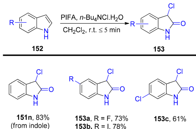
Scheme 63 Transformation of indole derivatives 152 into oxindole analogues 153 .
