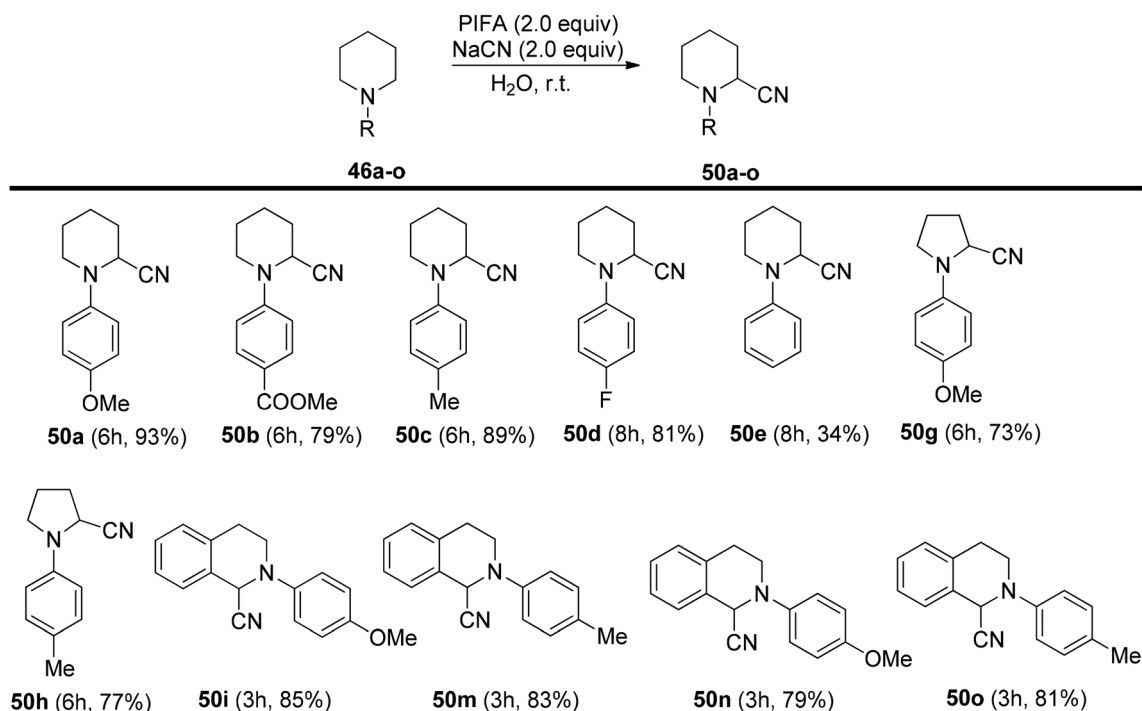
Scheme 19 Scope of cyanoation reaction.
