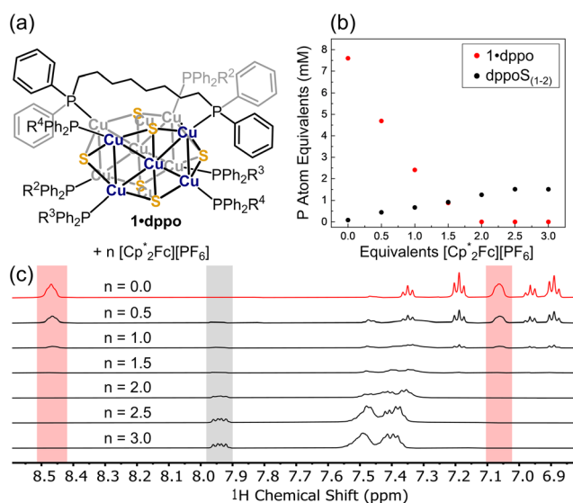
Fig. 5 (a) Reaction of 1-dppo with [\text{Cp}^*\text{Fe}][\text{PF}_6] (b) concentrations of 1-dppo (red trace) and phosphine sulfide products \text{dppoS}_{1-2} (black trace), expressed in terms of phosphorus atom equivalents, are plotted versus equivalents of [\text{Cp}^*\text{Fe}][\text{PF}_6] added. (c) ^1\text{H} NMR spectra (THF- d_8 , 400 MHz) collected for 1-dppo with n equivalents of [\text{Cp}^*\text{Fe}][\text{PF}_6] added. Diagnostic o-CH proton signals used to construct the plot in part (b) are highlighted for both 1-dppo (red) and phosphine sulfides \text{dppoS}_{1-2} (grey).
