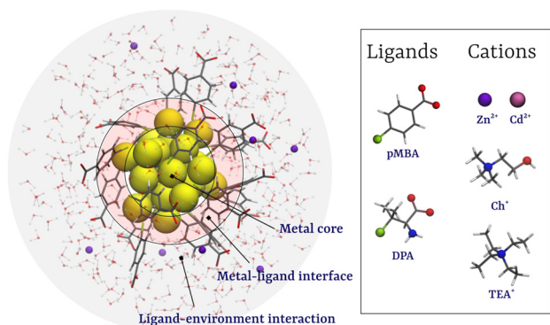
Fig. 1 Representation of an \text{Au}_{25}(\text{SR})_{18} MPC surrounded by the solvent (water) in the presence of cations. Ligands: para -mercaptobenzoic acid (pMBA) and D-penicillamine (DPA), divalent inorganic cations: \text{Zn}^{2+} and \text{Cd}^{2+} and monovalent molecular cations: cholinium ( \text{Ch}^+ ) and tetraethylammonium ( \text{TEA}^+ ).
