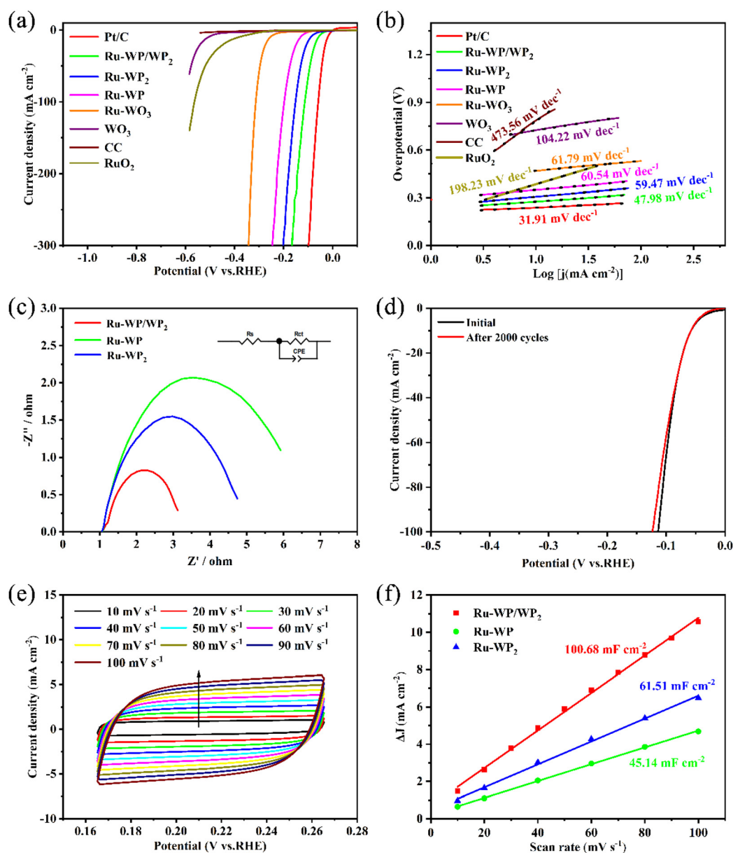
Fig. 4 Evaluation of the electrocatalytic hydrogen evolution activity of the catalyst in 0.5 M H_2SO_4 . (a) Linear sweep voltammetry curves of the catalysts at a scanning rate of 5 mV\ s^{-1} . (b) Tafel slope plots. (c) Nyquist fitting curves. (d) HER durability test. Polarization curve after 2000 cyclic voltammetry scans. (e) Cyclic voltammetry curves at different scanning rates (10–100 mV\ s^{-1} ). (f) The double-layer capacitance of the catalyst was calculated on the basis of the cyclic voltammetry curve.
