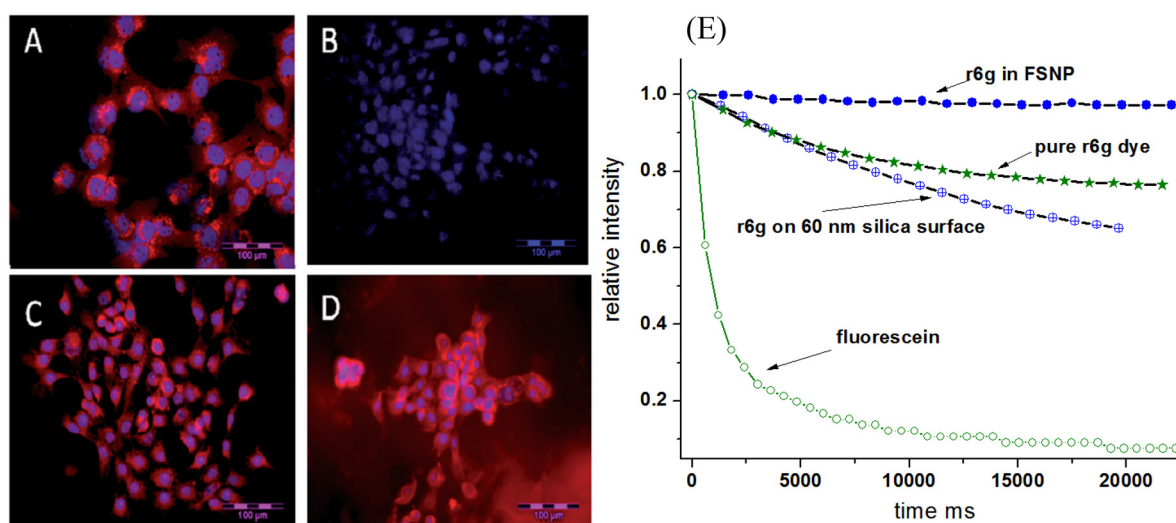
Fig. 3 Improved photobleaching of fluorescent dyes encapsulated in nano-UMSP. (A–D) NIR fluorescence microscopy of 4T1 luc tumor cells. (A) Cells 24 h post-treatment with LS277 dye; (B) re-imaging of cells shown in (A) after 9 weeks; (C) cells 24 h post-treatment with NP2_LS277 particles; (D) re-imaging of cells shown in (C) after 9 weeks; red: NIR fluorescence; blue: DAPI nuclear stain; scale bar 100 \mu\text{m} . (E) Photobleaching of rhodamine 6G dye, both free and encapsulated inside of mesoporous silica; the bleaching of the same dye physically adsorbed on solid silica nanoparticles is also shown. Photobleaching of fluorescein green dye of the same optical density is shown as a photobleaching standard. All photostability experiments were measured in aqueous environments. [Compiled using images taken from ref. 18 and 66. Reproduced from ref. 18 with permission from John Wiley and Sons, copyright 2008; Reproduced from ref. 66 with permission from RCS, copyright 2014].
