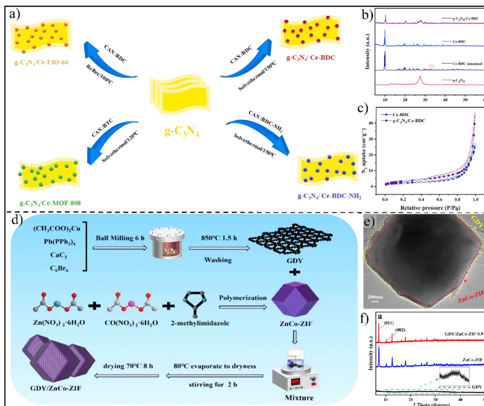
Fig. 8 (a) Synthesis process of g\text{-C}_3\text{N}_4/\text{Ce-MOF} . (b) XRD patterns of g\text{-C}_3\text{N}_4 , Ce-BDC, and g\text{-C}_3\text{N}_4/\text{Ce-BDC} . (c) \text{N}_2 adsorption–desorption isotherms of Ce-BDC and g\text{-C}_3\text{N}_4/\text{Ce-BDC} . Reprinted with permission from ref. 43. Copyright 2023 Elsevier. (d) Schematic for the preparation of GDY/ZnCo-ZIF. (e) TEM image of GDY/ZnCo-ZIF. (f) XRD spectra of GDY, ZnCo-ZIF and GDY/ZnCo-ZIF. Reprinted with permission from ref. 96. Copyright 2023 Elsevier.
