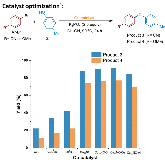
Fig. 4 Catalyst optimization. a Conditions: Ar–Br (0.3 mmol), 2 (0.375 mmol), Cu-catalyst used such as 5 mol% of CuCl or Cu t Bu-PPh 3 , Cu t Bu or 0.025 mol% of Cu 29 NC or Cu 29 -Celite S or Cu 29 NC-CeO 2 or Cu 29 NC-Al 2 O 3 , K 3 PO 4 (2.0 eq.), and acetonitrile (CH 3 CN) (2 mL). The mixture was stirred at 90 °C for 24 h. Yield refers to GC yield using 1,3,5-trimethylbenzene (mesitylene) as the internal standard.
