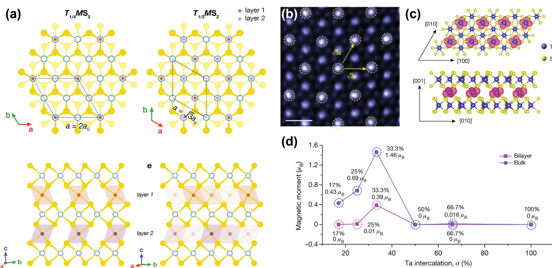
Fig. 4 Inducing magnetic order through transition metal intercalation. (a) Superlattices of Fe_xMS_2 and Cr_xMS_2 with M = Nb or Ta , for x = 1/4 and x = 1/3 . 134 (b) Atomic-resolution STEM-ADF (Scanning Transmission Electron Microscopy - Angular Dark Field) image of self-intercalated Ta_7S_{12} , showing the superstructure of the intercalated Ta ions. The scale bar corresponds to 0.5 nm. 135 (c) Top view (top) and side view (bottom) of the spin density isosurface of the intercalated Ta in Ta_7S_{12} . 135 (d) Calculated magnetic moments as a function of Ta intercalation ( \sigma ) in Ta_7S_{12} . 135 Reprinted with permission from ref. [134]. Copyright 2022 American Chemical Society. Reproduced from ref. [135] with permission from Springer Nature, copyright 2020.
