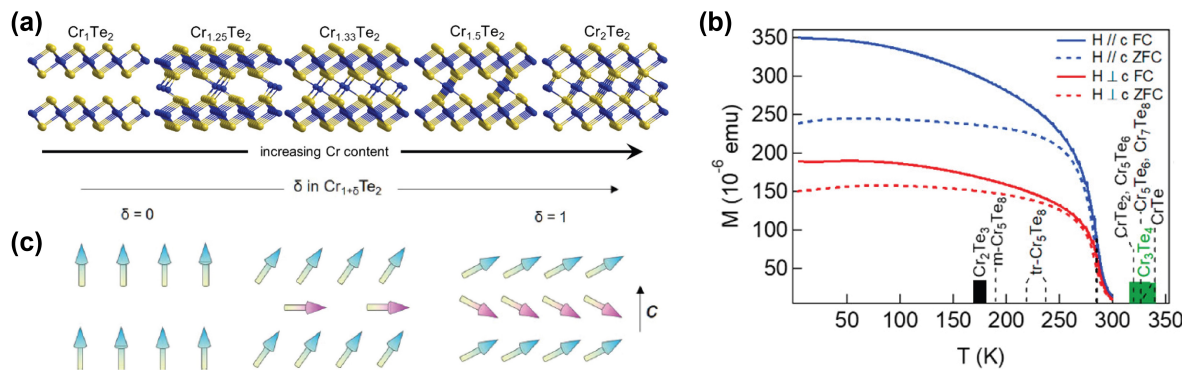
Fig. 3 Self-intercalation of CrTe 2 . (a) Crystal structures of CrTe 2 (Cr 1 Te 2 ), Cr 1.25 Te 2 (Cr 5 Te 8 ), Cr 1.33 Te 2 (Cr 2 Te 3 ), Cr 1.5 Te 2 (Cr 3 Te 4 ) and Cr 2 Te 2 (CrTe). 46 (b) Temperature-dependent magnetisation of Cr 1.5 Te 2 , also showing the ordering temperatures of various intercalation levels of CrTe 2 . 46 (c) Schematic drawing of the expected evolution of the ground-state magnetic configuration of Cr 1+δ Te 2 , with the arrows indicating the local spins. 115 Reprinted with permission from ref. [46]. Copyright 2021 American Chemical Society. Reprinted with permission from ref. [115]. Copyright 2020 by the American Physical Society.
