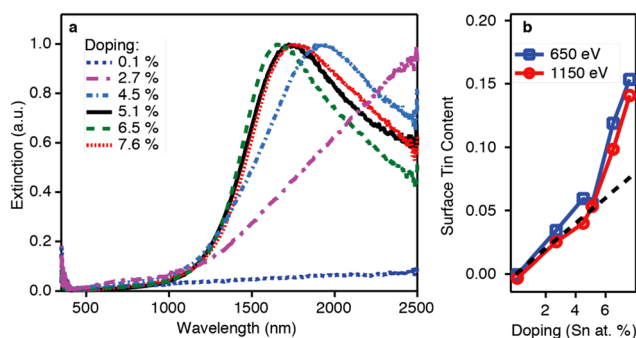
Fig. 11 (a) Optical extinction and (b) XPS depth profiling versus the doping series. The dotted black line in panel (b) shows the expected \text{Sn}/(\text{In} + \text{Sn}) ratio for a uniform doping profile. Reproduced from ref. 51 with permission from ACS, copyright 2014.
