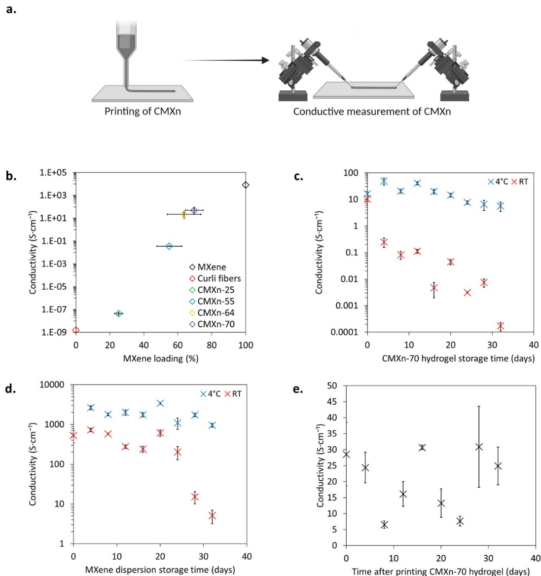
Figure 5. Conductivity of printed CMXn hydrogels over time. (a) Schematic of conductivity measurements at RT & 45% relative humidity (RH) for printed CMXn hydrogels, followed by (b) conductivity measurements of CMXn hydrogels plotted as a function of their MXene load, (c) shelf life of CMXn-70 hydrogel at refrigerated (4°C) and RT conditions, (d) shelf life of MXene dispersion at 4°C and RT & (e) stability of printed CMXn-70 hydrogel.
