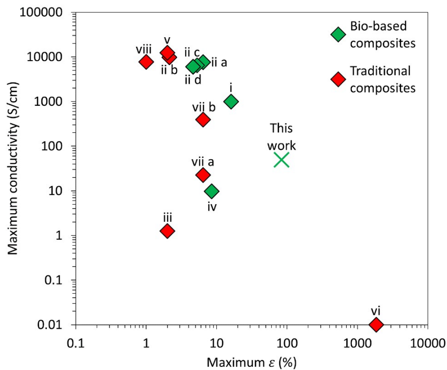
Figure 6. Comparison of maximum ultimate strain ( \epsilon ) and maximum conductivity achieved by other MXene composite films using different manufacturing techniques. Nomenclature and numerical values are shown in Table S1 . Further mechanical properties and assembly techniques are shown in Table S2 .
