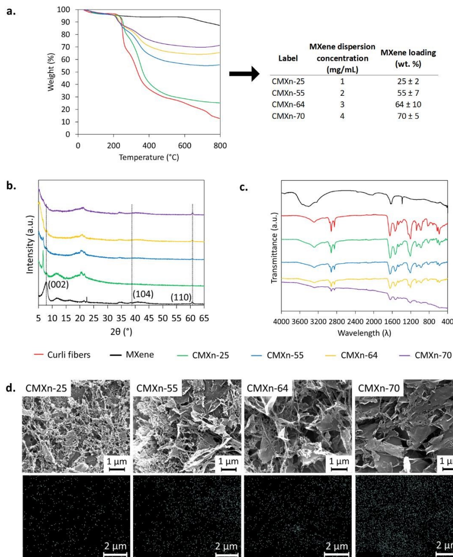
Figure 2. MXene loading in CMXn hydrogels varies with the concentrations of MXene dispersions ranging from 1 to 4 mg/mL, after incubation with curli fibers. Assessment of the loading through (a) TGA with table that correlates MXene dispersions used and their corresponding loading weights in CMXn hydrogels. The nanocomposites were labelled according to their MXene loading content, (b) XRD, (c) FTIR spectroscopy, and (d) SEM images of CMXn hydrogels with corresponding EDS elemental mapping for Ti.
