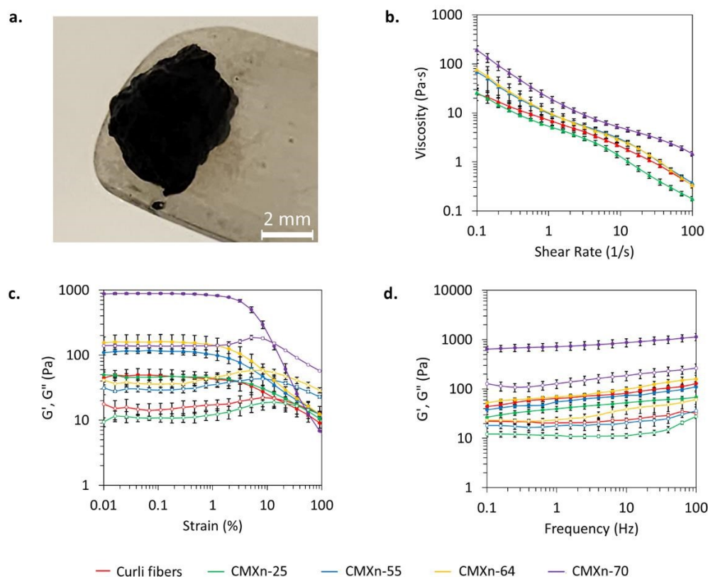
Figure 3. Rheological properties of CMXn hydrogels. All measurements were done with the nanocomposites in their hydrated state: (a) close-up image of CMXn-70 hydrogel, (b) viscosity as a function of shear rate (solid triangle markers), storage ( G' ) and loss ( G'' ) modulus (solid and empty circles, respectively) under (c) amplitude & (d) frequency sweeps.
