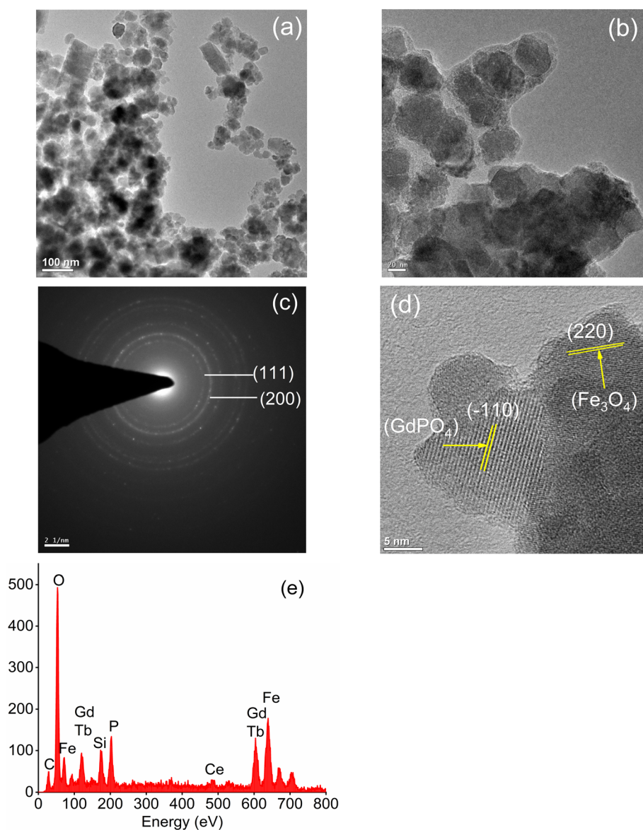
Fig. 2 TEM images of (a) \text{Fe}_3\text{O}_4 nanoparticles and (b) CMC functionalized \text{Fe}_3\text{O}_4@SiO_2@GdPO_4:Tb^{3+},Ce^{3+} nanocomposites. (c) SAED pattern of \text{Fe}_3\text{O}_4 nanoparticles, (d) HRTEM image and (e) EDS spectra of CMC functionalized \text{Fe}_3\text{O}_4@SiO_2@GdPO_4:Tb^{3+},Ce^{3+} nanocomposites.
