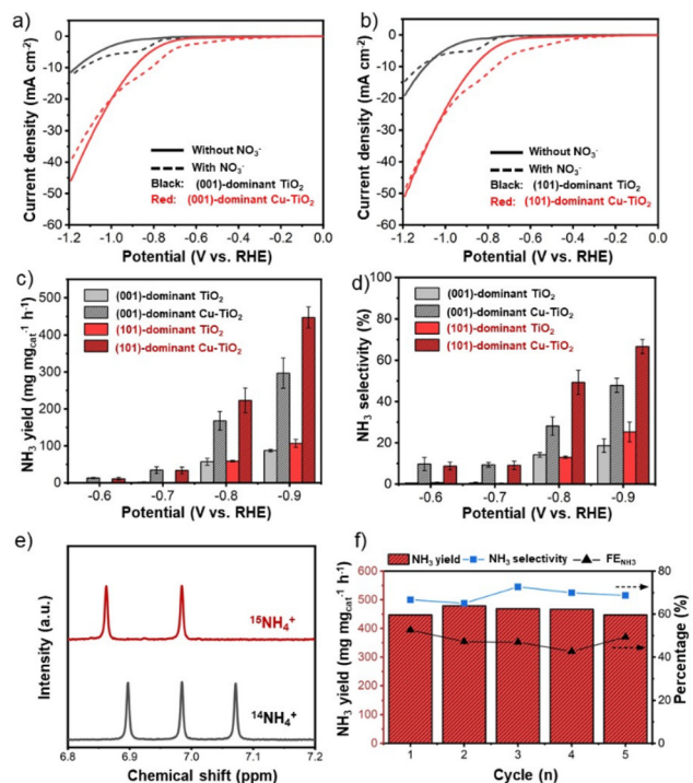
Fig. 3 LSV curves of (a) the (001)-dominant \text{TiO}_2 and (001)-dominant \text{Cu-TiO}_2 , and (b) the (101)-dominant \text{TiO}_2 and (101)-dominant \text{Cu-TiO}_2 in 0.5 M \text{Na}_2\text{SO}_4 without and with the addition of 50 ppm \text{NO}_3^- -N. (c) \text{NH}_3 yield and (d) \text{NH}_3 selectivity. All catalytic activity experiments were performed in 0.5 M \text{Na}_2\text{SO}_4 containing 50 ppm \text{NO}_3^- -N. (e) ^1\text{H} NMR spectra of the electrolyte after the electrocatalytic reduction reaction using ^{15}\text{NO}_3^- and ^{14}\text{NO}_3^- as the nitrogen sources. The reaction for isotope labelling was performed for the (101)-dominant \text{Cu-TiO}_2 at -0.9 V vs. RHE in 0.5 M \text{Na}_2\text{SO}_4 containing 50 ppm \text{NO}_3^- -N. (f) Stability test of the (101)-dominant \text{Cu-TiO}_2 was performed at -0.9 V vs. RHE in 0.5 M \text{Na}_2\text{SO}_4 containing 50 ppm \text{NO}_3^- -N.
