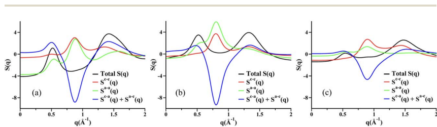
Fig. 2 Cation–cation, anion–anion, cation–anion, and total simulated S(q) for (a) N_{5,5,5,5}^+/\Gamma^- , (b) N_{5,5,5,5}^+/PF_6^- , and (c) N_{5,5,5,5}^+/N(CN)_2^- in the liquid state. Reprinted 15 (adapted) with permission from J. Phys. Chem. Lett. , 2013, 4(1), 105–110. Copyright 2013 American Chemical Society.
