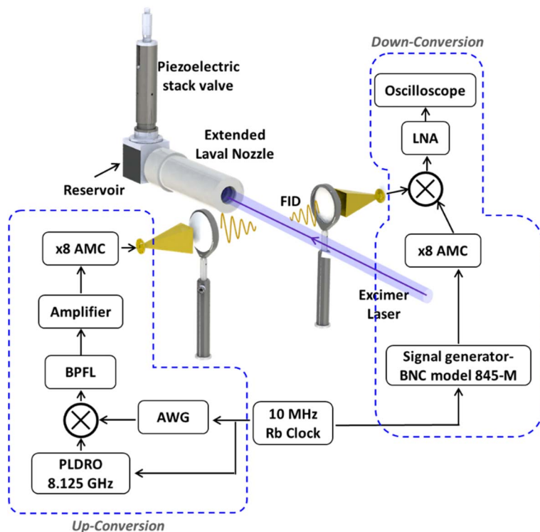
Fig. 1 Schematic illustration of the main components of the CUPF experiment.
