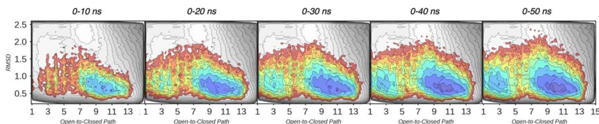
Fig. 4 Estimated FEL of OB2-PfTrpB . The estimated FEL from the accumulated multiple replica nanosecond timescale MD simulations performed starting at the ensemble of template-based AF2 predictions, is shown in colour on top of the previously reconstructed FEL of the PfTrpB variant (shown in grey scale). 19 FELs are displayed every 10 ns of MD simulation time and using two different combinations of forcefield and water model: (A) ff14SB and TIP3P water, and (B) ff19SB and OPC water. The x axis denotes the ensemble of structures generated from X-ray data for the open-to-closed transition of the COMM domain, which ranges from 1–5 (open, O), 6–10 (partially closed, PC), to 11–15 (closed, C), the y axis is the mean square deviation (MSD, in Å 2 ) from the path of O-to-C structures generated. Most stable conformations are shown in blue, whereas higher energy regions are shown in red.
