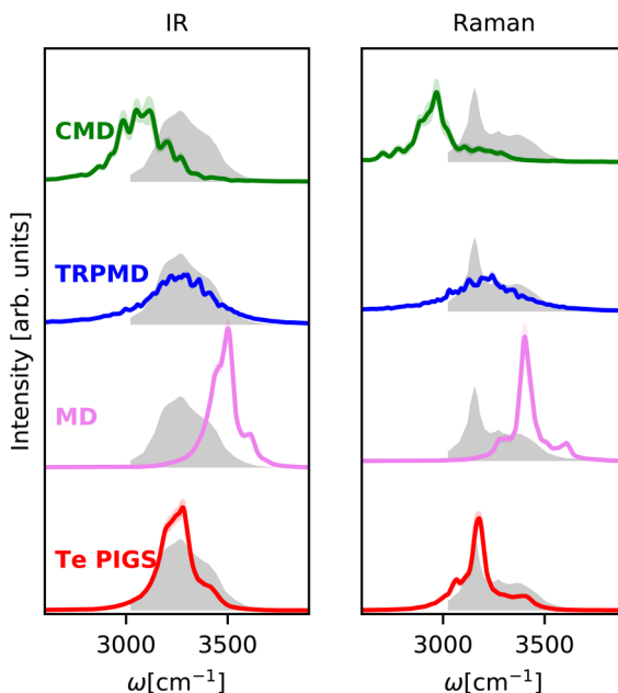
Fig. 3 IR and Raman stretching band of polycrystalline ice at 150 K with the T_e PIGS (red), MD (pink), TRPMD (blue), and CMD (green) and the experimental spectra 92 (shifted by 22 cm -1 to account for the missing quantum coherence effects in simulation methods) in grey. All simulations are performed with a BPNN with SPC charges trained at the revPBE0-D3 level of theory.
