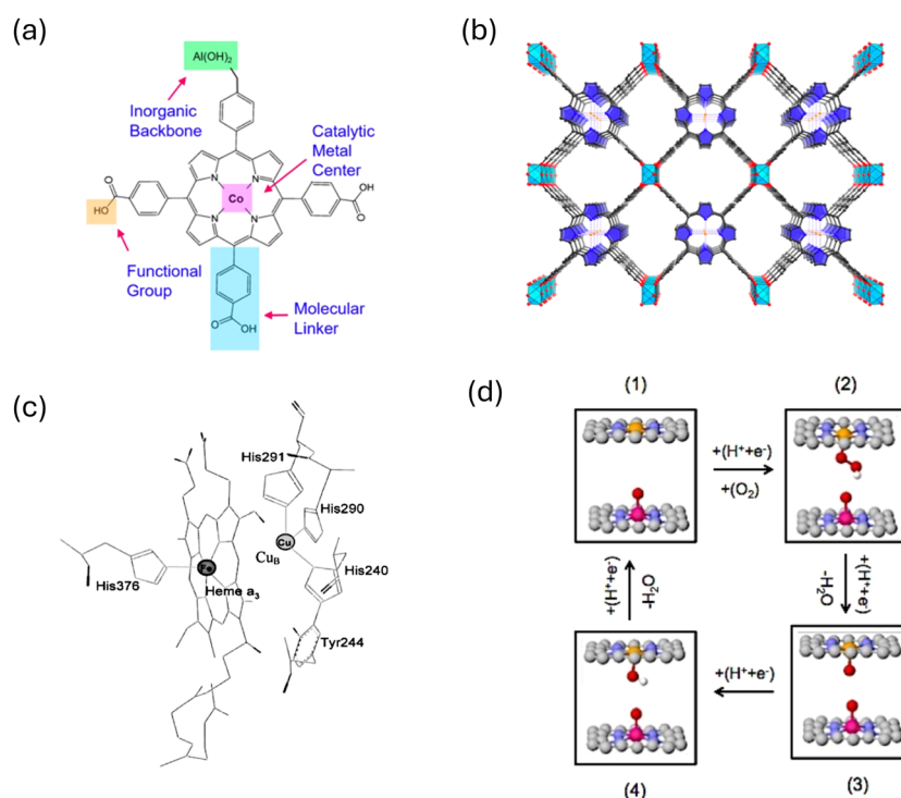
Fig. 5 (a) and (b) Coordination entity for constructing \text{Al}_2(\text{OH})_2\text{TCCPP-Co} MOF. Adapted from ref. 55 with permission. (c) Cytochrome- C oxidase enzyme. Adapted from ref. 58 with permission. (d) Illustration of the bio-mimic prototype catalyst capable of circumventing the scaling relations.
