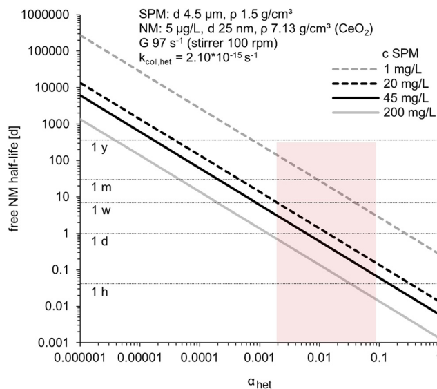
Fig. 5 Pseudo-first-order free NM half-life in dependence of \alpha_{\text{het}} calculated for different SPM concentrations ( c_{\text{SPM}} : 1, 20, 45, 200 mg L -1 ) setting the parameters to represent the experiments ( i.e. , for SPM: diameter 4.5 \mu\text{m} , density 1.5 g cm -3 ; for NM: concentration 5 \mu\text{g L}^{-1} , diameter 25 nm, density of CeO 2 7.13 g cm -3 ; assuming spherical shape for both; velocity gradient G 97 s -1 for 100 rpm stirring). Black lines indicate the SPM concentrations used in the experiments, and the shaded area highlights the range of \alpha_{\text{het\_size-dis}} values determined (see Fig. 3).
