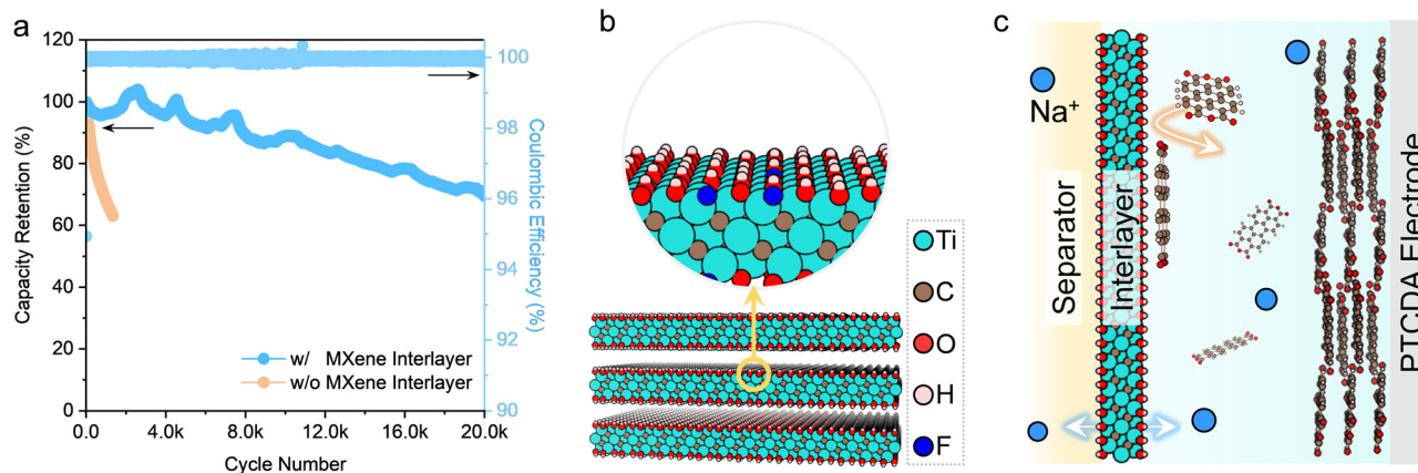
Fig. 5 Cycling stability tests. Cycling stability of the PTCD A electrode in the hybrid electrolyte ( n_{\text{NaClO}_4} : n_{\text{acetamide}} : n_{\text{water}} = 1 : 4 : 4 ) with and without the MXene interlayer (current rate: 100C). Schemes of the 2D MXene nanosheets with negatively charged surfaces (b) and a cell configuration with the MXene interlayer to mitigate the dissolution of PTCD A during operation (c).
