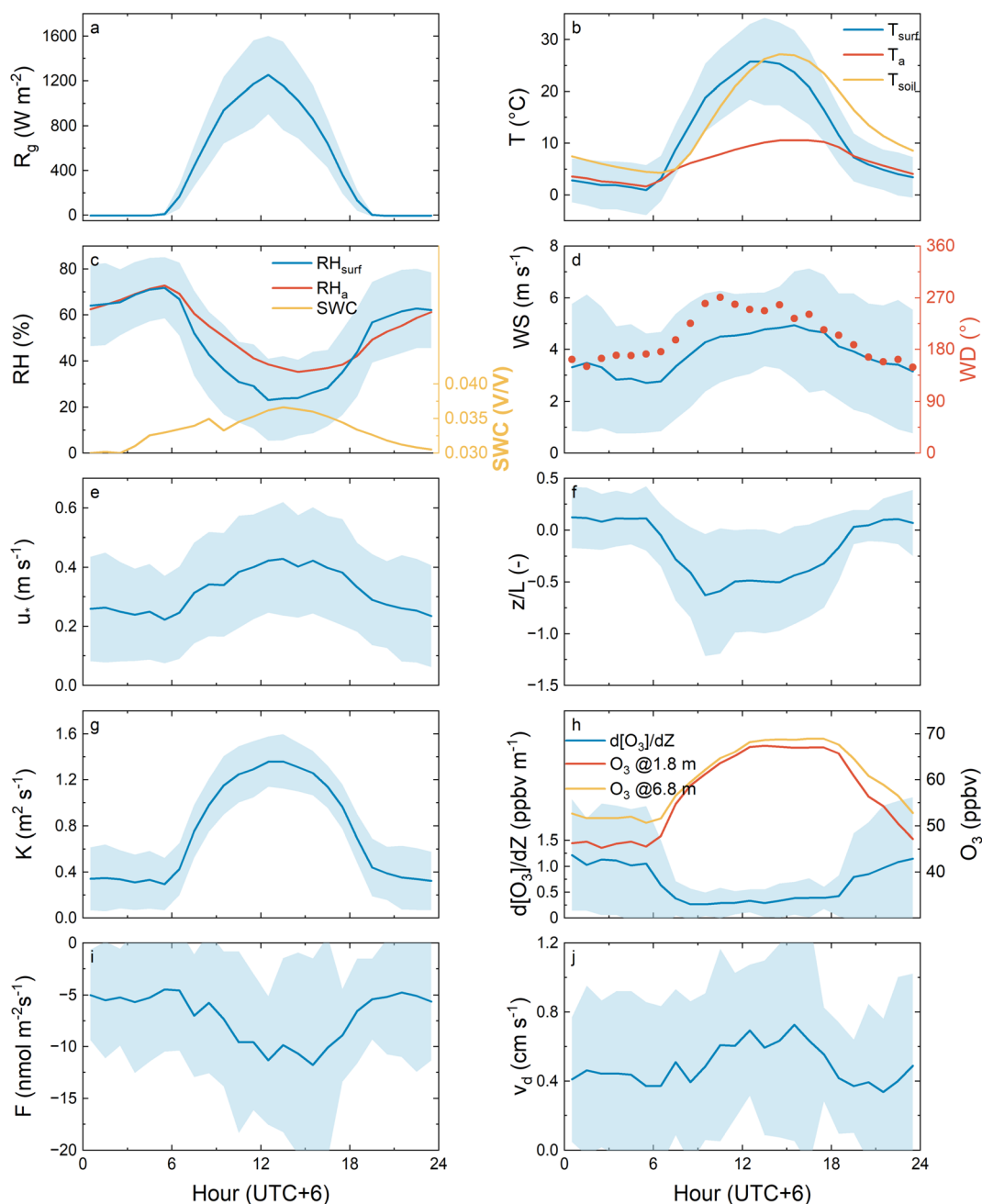
Fig. 2 Diel pattern of meteorological parameters and edaphic parameters associated with ozone velocity derivation and deposition resistance derivation. Diel pattern of (a) solar radiation ( R_g ), (b) air temperature at 1.8 m ( T_a ), surface temperature ( T_{surf} ) and soil temperature at -5 cm ( T_{soil} ), (c) air relative humidity at 1.8 m ( RH_a ), surface relative humidity ( RH_{surf} ) and soil water content (SWC), (d) wind speed at 1.8 m (WS) and wind direction (WD), (e) friction velocity ( u_* ), (f) atmospheric stability criterion ( z/L ), (g) turbulence exchange coefficient ( K ), (h) gradient of ozone between 6.8 m and 1.8 m ( d[O_3]/dZ ), ozone concentration at 6.8 m and ozone concentration at 1.8 m, (i) ozone flux ( F ), and (j) ozone deposition velocity ( v_d ). The solid line is the diel mean, and the shading is variation of our observations.
