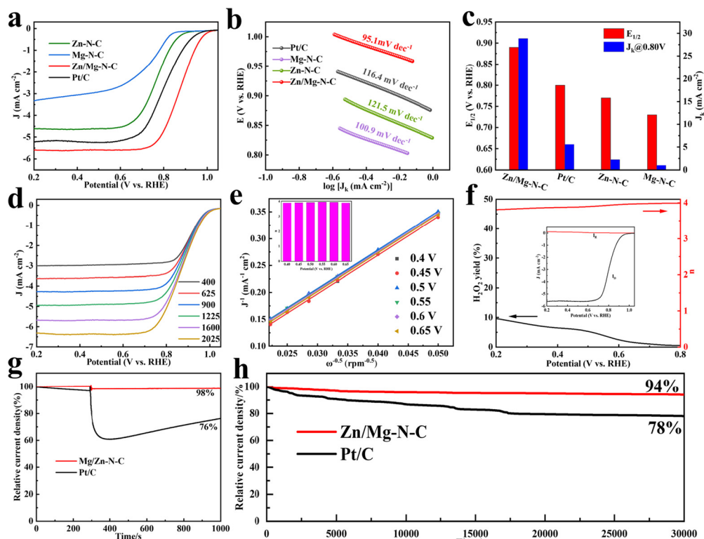
Fig. 3 LSV curves of Zn/Mg–N–C, Zn–N–C, Mg–N–C and Pt/C catalysts in O_2 -saturated 0.1 M KOH (rotation rate: 1600 rpm; sweep rate: 10 mV s^{-1} ). (b) Tafel plots of the investigated catalysts. (c) The kinetic current density ( J_k ) at 0.8 V and E_{1/2} of the catalysts. (d) LSV curves of Zn/Mg–N–C at various rotation speeds. (e) K–L plots and electron transfer numbers of Zn/Mg–N–C. (f) H_2O_2 yield and electron transfer number ( n ) from the RRDE measurement of Zn/Mg–N–C in O_2 -saturated 0.1 M KOH at 1600 rpm (inset: the corresponding RRDE voltammograms). (g) Methanol tolerance test for Zn/Mg–N–C and Pt/C. (h) Long-term stability of Zn/Mg–N–C and Pt/C.
