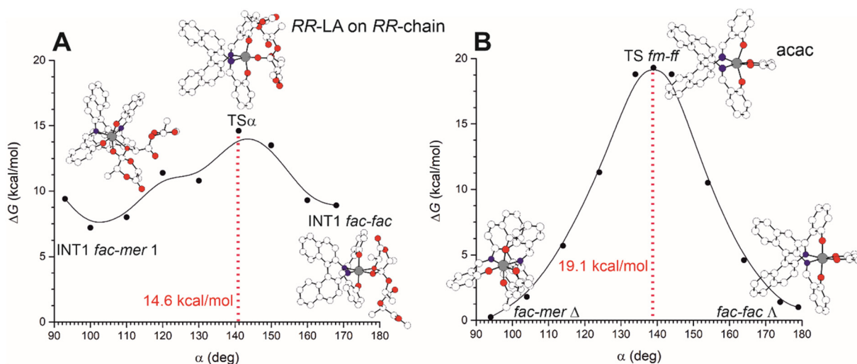
Fig. 4 Free energy profiles of the transformation from fac-mer \Delta to fac-fac \Lambda for ( R )-1 as a function of the O_L-Al-O_L valence bond. The reorganization path moving from TS1 ( fm1 ) to TS2 ( ff ) as a function of \alpha for RR -LA polymerization is reported in A. The analogous path by using the bidentate acac − is reported in B. Aluminum, oxygen and nitrogen atoms in gray, red and blue. Hydrogen atoms have been omitted for clarity.
