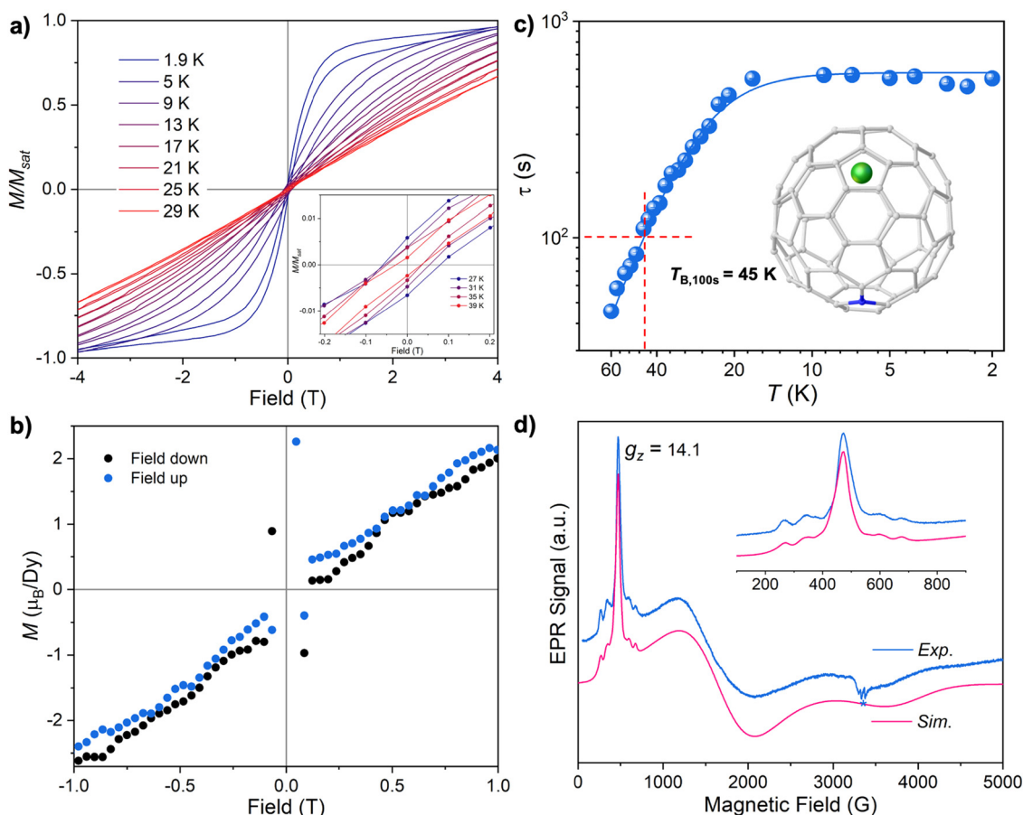
Fig. 8 (a) Magnetic hysteresis loops for \text{Dy}@C_{81}\text{N} at 1.9–39 K using SQUID magnetometry with a field sweep rate of 3.5\text{ mT s}^{-1} . (b) Magnetic hysteresis for \text{Dy}@C_{81}\text{N} at 5 K recorded by using the XMCD technique. (c) Temperature-dependence of magnetization relaxation times for \text{Dy}@C_{81}\text{N} and the determination of its blocking temperature T_{\text{B},100\text{s}} = 45\text{ K} . The inset shows its molecular structure. (d) Experimental and simulated EPR spectra of \text{Dy}@C_{81}\text{N} in a toluene solution at 10 K. The inset illustrates the hyperfine structures. Reproduced from ref. 16.
