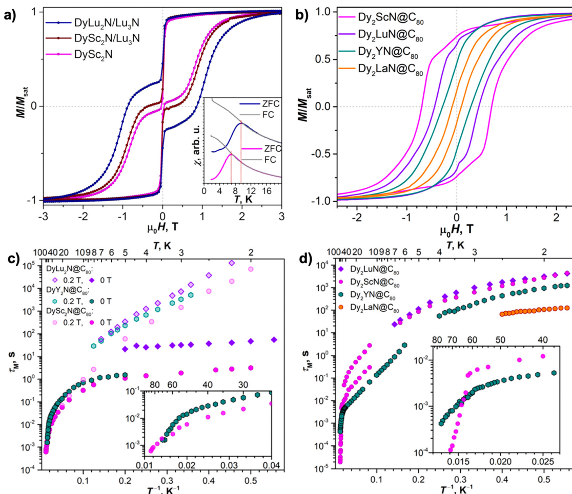
Fig. 3 (a) Magnetic hysteresis loops of \text{DyLu}_2\text{N}@C_{80} measured at 2 K and compared with those of \text{DySc}_2\text{N}@C_{80} and \text{DySc}_2\text{N}@C_{80} diluted with \text{Lu}_3\text{N}@C_{80} in a 1:1 ratio. Sweep rate: 2.9 \text{ mT s}^{-1} . The inset shows the determination of the bifurcation temperature, T_{\text{B,ZFC}} , from the temperature dependence of the magnetic susceptibility with a temperature sweep rate of 5 \text{ K min}^{-1} . (b) Magnetic hysteresis loops for \text{Dy}_2\text{MN}@C_{80} ( M = \text{Sc}, \text{Y}, \text{La}, \text{Lu} ) at 2 K (2.1 K for the La case) with a field sweep rate of 2.9 \text{ mT s}^{-1} . (c) and (d) Magnetization relaxation times of \text{DyM}_2\text{N}@C_{80} ( M = \text{Sc}, \text{Y}, \text{Lu} ) (c) and of \text{Dy}_2\text{MN}@C_{80} ( M = \text{Sc}, \text{Y}, \text{La}, \text{Lu} ) (d). The insets in (c) and (d) show enlargement of high-temperature parts. Reproduced from (a) ref. 78 and (b)–(d) ref. 79.
