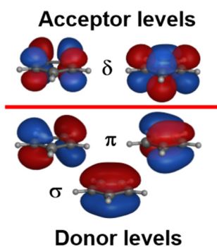
Fig. 7 Schematic MO plots of valence \pi orbitals for \text{Cp}^- .
