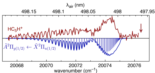
Fig. 5 REPD spectrum of the \text{HC}_5\text{H}^+ \tilde{\text{A}}^2\Pi_{\text{g}}(1/2) \leftarrow \tilde{\text{X}}^2\Pi_{\text{u}}(1/2) band origin measured using a dye laser (bandwidth 0.04\text{ cm}^{-1} ). The spectrum is compared with a simulation generated using B'' = 0.07477\text{ cm}^{-1} , B' = 0.07193\text{ cm}^{-1} , and T = 12\text{ K} . The vertical arrow indicates the position of the 497.961\text{ nm} DIB (data from ref. 62).
