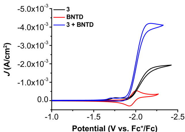
Fig. 3 CVs of 1.0 mM \text{Cr}(\text{t}^{\text{bu}}\text{d}^{\text{h}}\text{t}^{\text{bu}}\text{bpy})\text{Cl}(\text{H}_2\text{O}) 3 and 2.5 mM BNTD alone and together under \text{CO}_2 saturation conditions with 0.5 M PhOH in DMF demonstrating the shift in catalytic potential.
