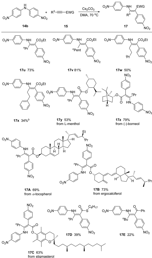
Scheme 3 Scope of alkyne. a 14b (1.2 equiv.), 15 (1.0 equiv.) and \text{Cs}_2\text{CO}_3 (1.5 equiv.) in DMA at 70^\circ\text{C} .
