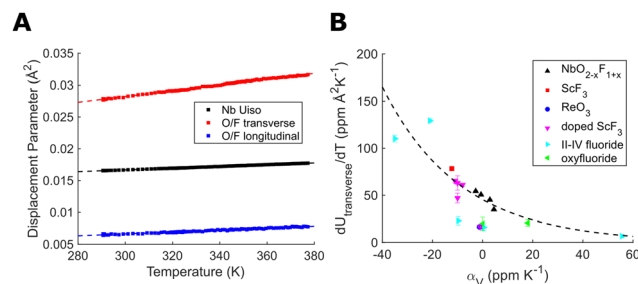
Fig. 3 (A) Refined displacement parameters for \text{NbO}_2\text{F} . (B) The gradient of the transverse displacement parameter in \text{ReO}_3 -type structures showing its relationship with mean volumetric CTE. 14,15,19,25,29–33 Linear fits were performed over the full temperature range of data available for which the structure remains cubic.
