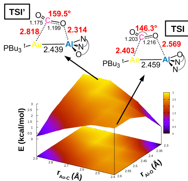
Fig. 4 Potential energy surface (PES) in the region surrounding transition state TSI for complex [\text{Bu}_3\text{PAuAl}(\text{NON})] . Insets: Position on the PES and schematic structure of TSI and TSI'. Energy has been shifted in each case according to the minimum energy structure. Reproduced with permission from ref. 39 Copyright 2022, American Chemical Society.
