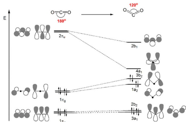
Scheme 4 Qualitative Walsh diagram for the OCO angle bending from 180^\circ to 120^\circ . Most important frontier molecular orbitals of \text{CO}_2 are depicted.
