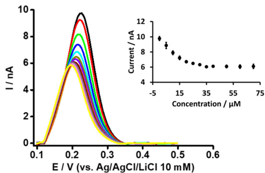
Fig. 4 DPVs at different concentrations of \beta -CD at a fixed concentration of PFOA ( 5 \mu\text{M} ) at the \mu TIIES array. Cell composition as shown in Scheme 1. Black, red, green, blue, cyan, dark yellow, violet, orange, wine red, gray, magenta, and yellow, respectively, represent the DPVs at 0, 5, 10, 15, 20, 25, 30, 35, 40, 50, 60, and 70 \mu\text{M} \beta -CD. Inset: relationship between current and concentration of \beta -CD. DPVs are background-subtracted followed by baseline-corrected. Error bars indicate \pm 1 standard deviation from three independent measurements.
