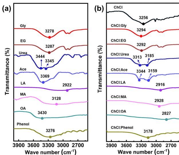
Fig. 2 FTIR spectra of the DESs tested in the range of 4000–2500 cm -1 . (a) FTIR spectra for the 8 pristine HBAs. (b) FTIR spectra of the pristine ChCl as the HBA and the corresponding DESs with the molar ratio of 1 HBA : 2 HBD.
