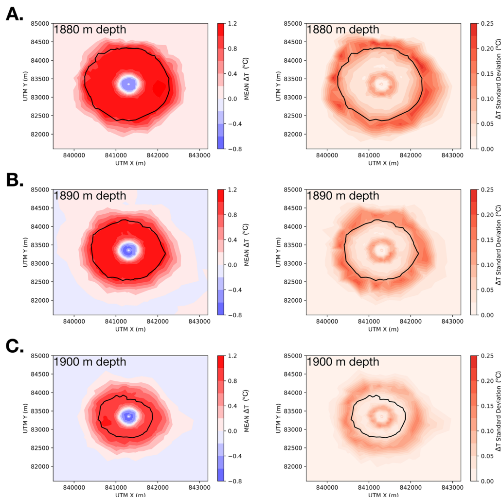
Fig. 9 Ensemble simulation results ( N = 50 ) of temperature changes ( \Delta T °C) within the injection reservoir after 10 years of CO 2 injection at (A) 1880 m depth, (B) 1890 m depth, and (C) 1900 m depth. The black contour indicates the furthest extent of the free-phase CO 2 plume, defined as the mean 1% CO 2 saturation contour (Fig. 7). Mean \Delta T is shown on the left column with the corresponding standard deviation on the right. Note that the max temperature drop ( -\Delta T ) is -0.8 °C near the injection well (left column, blue shading) and temperature increase ( +\Delta T ) is +1.2 °C (left column, red shading). Also note that the lateral extent of the temperature change in the reservoir is greater than the lateral extent of the CO 2 plume (black contour).
