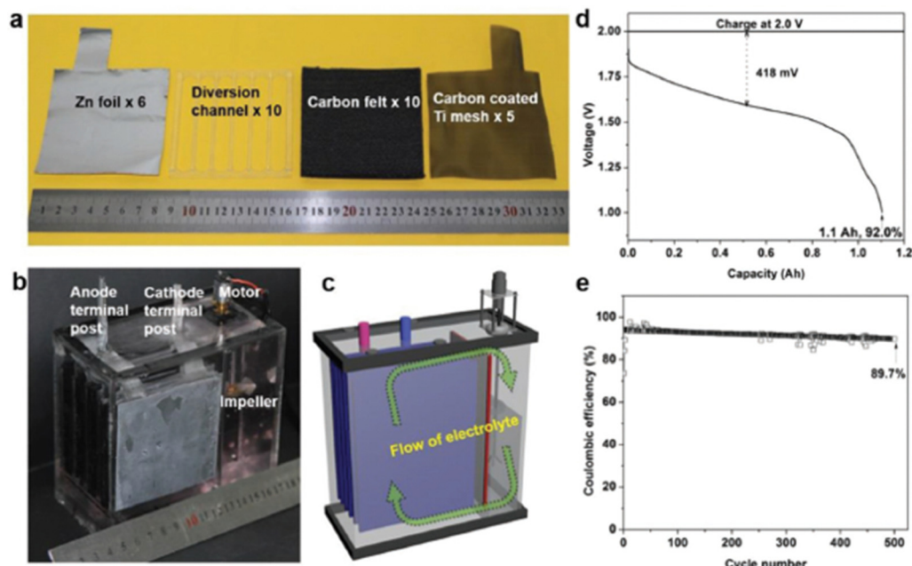
Fig. 15 (a) The cell components used for the membrane free aqueous Zn/MnO 2 RFB, (b) photographic image of the Zn/MnO 2 RFB, (c) schematic diagram of the indication of electrolyte flow, (d) the GCD profile of the Zn/MnO 2 RFB, and (e) the cyclability of the Zn/MnO 2 RFB (reproduced from ref. 87 with permission from Wiley).
