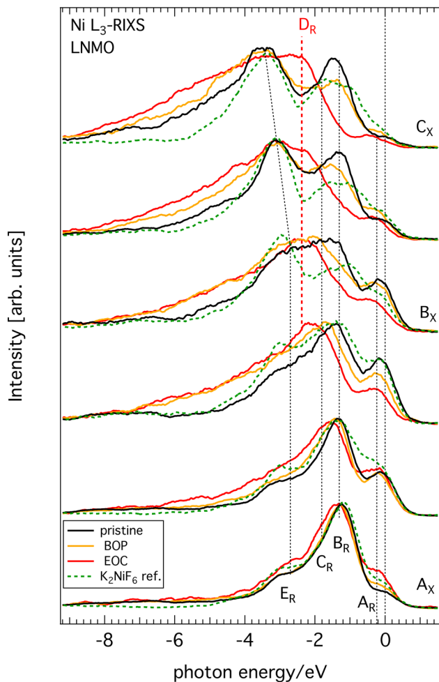
Fig. 5 RIXS spectra across the Ni L_3 -resonances A_x , B_x , C_x of Li_{1-x}Ni_{0.44}Mn_{1.56}O_4 from three selected SoCs and from the Ni(IV) reference compound K_2NiF_6 (see color coded legend). Each spectrum is normalized to its respective maximum to facilitate spectral shape comparison.
