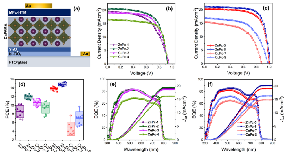
Fig. 6 Proposed device architecture: fluorine-doped tin oxide (FTO)/bi-TiO 2 /SnO 2 /perovskite/MPc/Au (a), J - V curves of the device using (b) symmetric MPcs and (c) asymmetric MPcs, (d) statistical PCE of PSCs with different MPc-HTMs, corresponding IPCE and integrated current density ( J_{\text{int}} ) of the device with (e) symmetric MPcs and, (f) asymmetric MPcs.
