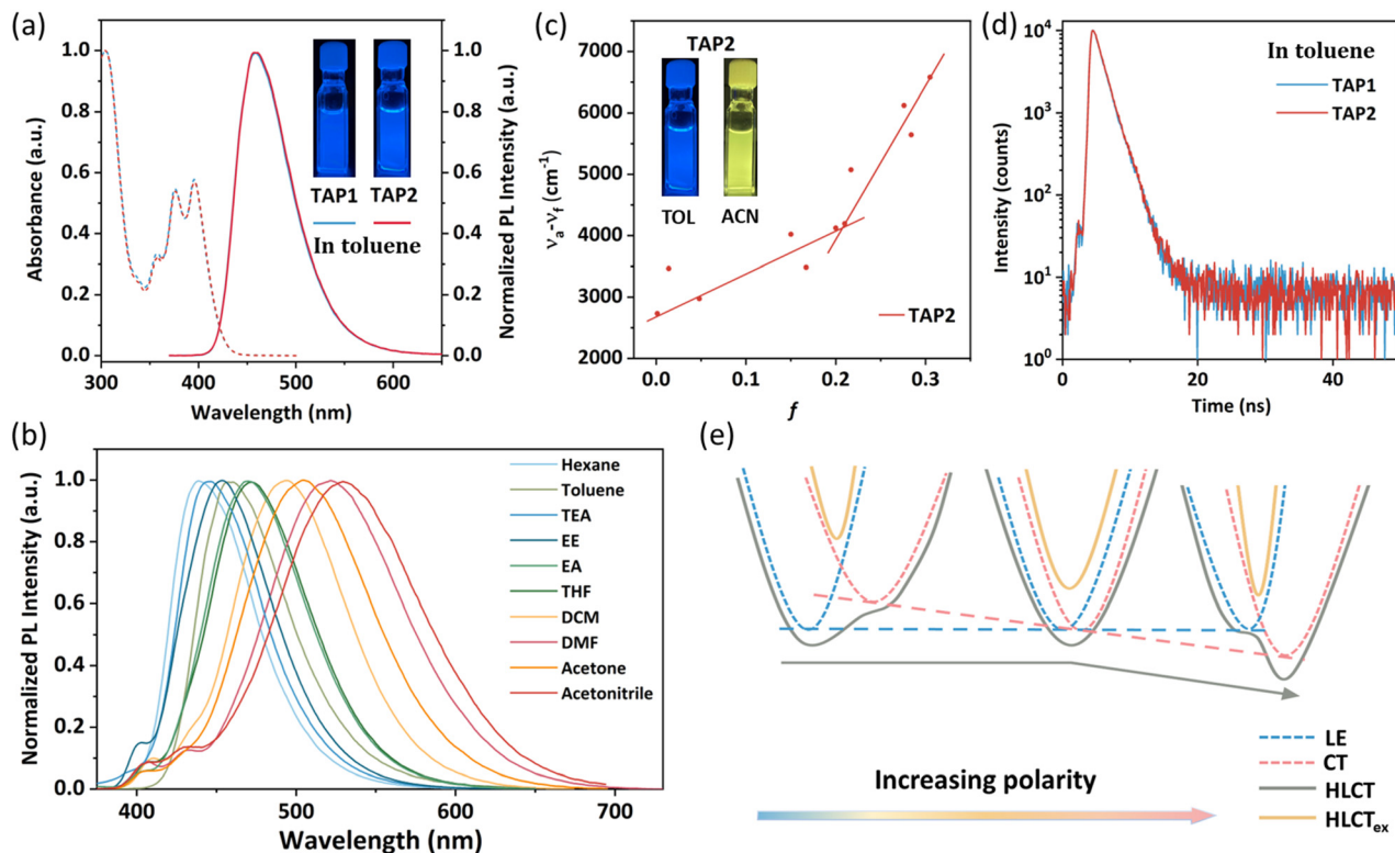
Fig. 2 (a) UV-vis absorption and PL spectra of TAP1 and TAP2 in toluene ( 10^{-5} mol \text{L}^{-1} ). Insets show photographs of TAP1 and TAP2 in dilute toluene under 365 nm excitation. (b) PL spectrum of TAP2 in different solvents under 355 nm excitation. (c) Solvatochromic Lippert–Mataga models of TAP2 under 355 nm excitation. Insets show photographs of TAP2 in dilute toluene (left) and acetonitrile (right) under 365 nm excitation. (d) Lifetime decay curves of TAP1 and TAP2 in toluene ( 10^{-5} mol \text{L}^{-1} ). (e) Illustration of HLCT state formation in solvents with different polarities.
