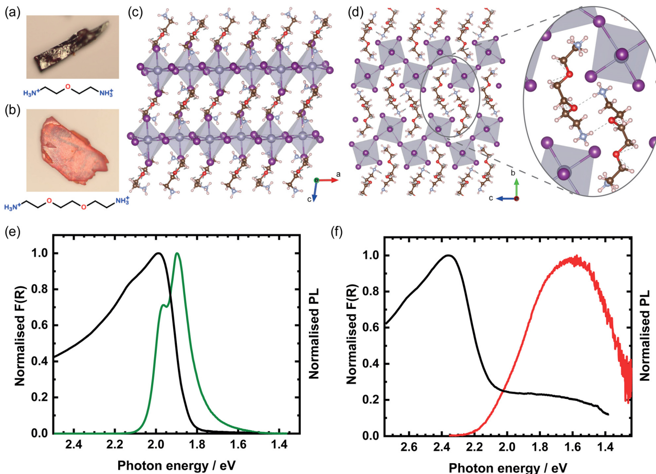
Fig. 1 (a) OBESnI 4 and (b) EDBESnI 4 images of mm-sized single crystals. Crystal structure of (c) OBESnI 4 and (d) EDBESnI 4 , where grey atoms are Sn, purple are I, blue are N, brown are C, red are O, and white are H. The inset highlights the formed hydrogen bonds. Kubelka–Munk transformed diffuse reflectance and photoluminescence spectra of (e) OBESnI 4 and (f) EDBESnI 4 .
