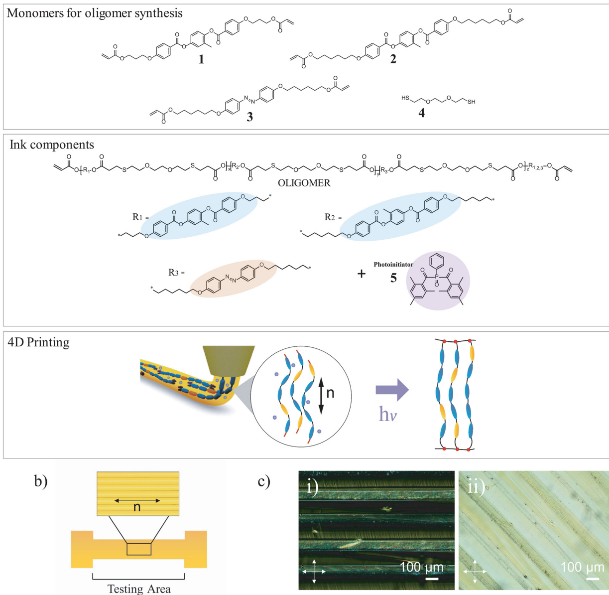
Fig. 1 (a) (top box) Molecular structure of the components to prepare the oligomer: diacrylate mesogens RM257 (1) and RM82 (2), diacrylate azobenzene A6A (3) and dithiol chain extender DODT (4). Blue elongated ovals represent the rigid core of the reactive mesogens, while orange ones represent that of the pro-mesogenic azobenzene. The purple circle represents the non-mesogenic photoinitiator. (Middle box) Ink components including the oligomer and the Irgacure 819 photoinitiator (5). The oligomer was synthesized via a base-catalyzed thiol-acrylate Michael addition reaction of the reactive mesogens and DODT. Mole ratios were 2.275 : 2.275 : 0.45 : 4.5 for RM82 : RM257 : A6A : DODT; photoinitiator (5) was added to the ink at a proportion of 2 wt%. (Bottom box) Ink printing and photocrosslinking of oligomers turning into a LCE. (b) Cartoon illustration of the geometry and printing direction of the samples, along the yellow lines, defining the director n (two-headed arrow). (c) POM images of the printed sample consistent in closely printed lines leading to a continuous strip. POM images were acquired between crossed polarizers (crosses indicate polarizer transmission directions) with the printing direction oriented (i) at 0^\circ and (ii) at 45^\circ with respect to the first polarizer transmission direction (scale bar = 100 \mu\text{m} ).
