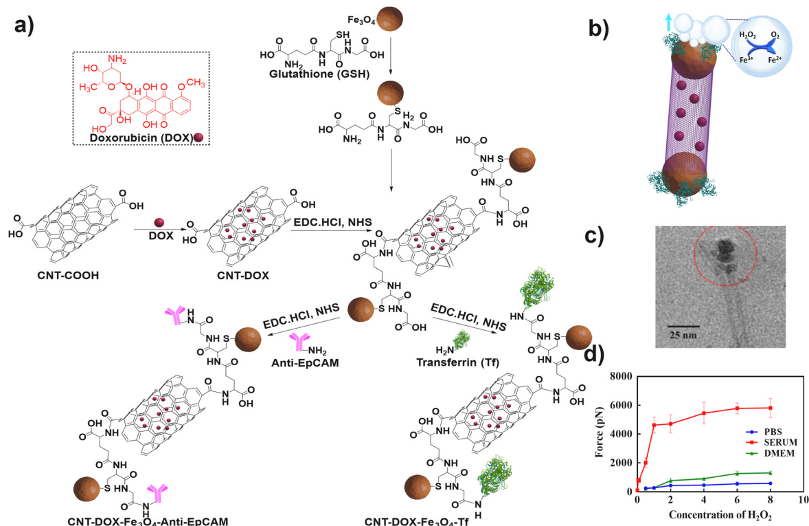
Fig. 5 (a) Steps involved in the synthesis of CNT-DOX- \text{Fe}_3\text{O}_4 -Tf or CNT-DOX- \text{Fe}_3\text{O}_4 -EpCAM nanobots. Information adapted from ref. 31. (b) Reaction mechanism involved in the propulsion of CNT-DOX- \text{Fe}_3\text{O}_4 -Tf nanobots. Information adapted from ref. 31. (c) TEM micrograph of the CNT-DOX- \text{Fe}_3\text{O}_4 -Tf nanobot. Red circle indicates the \text{Fe}_3\text{O}_4 capped end of the CNT. Reproduced from ref. 31. (d) Graphical representation of alterations in the force generated during the propulsion of nanobots in various media. Reproduced from ref. 31.
