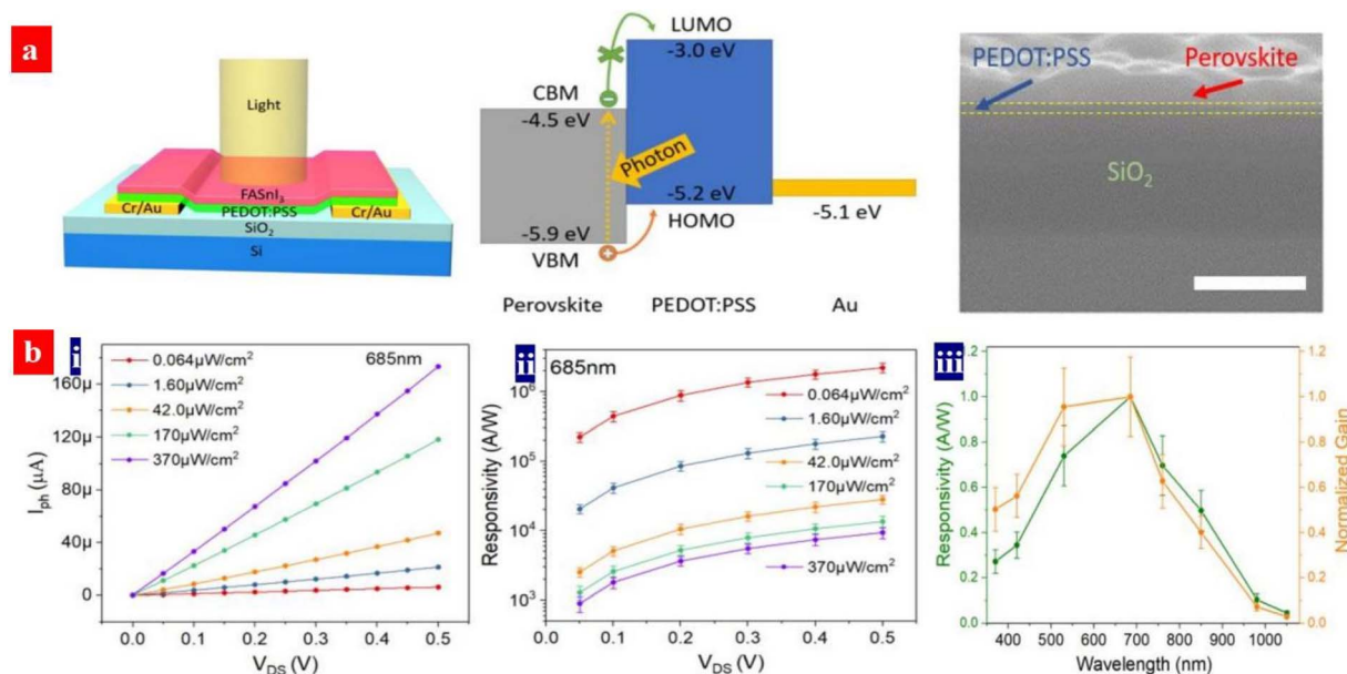
Fig. 11 (a) Architecture structure of the PDs, energy band diagram, and cross-sectional SEM image of (a) FASn 13 /PEDOT:PSS bilayer coated on SiO 2 /Si. Scale bar: 300 nm. (b) (i) Photo-current vs. drain voltage; (ii) average responsivity vs. drain voltage under various intensity of light. Wavelength: 685 nm; and (iii) normalized spectral responsivity and gain of the PD. Reproduced with permission. 157 Copyright 2020, American Chemical Society.
