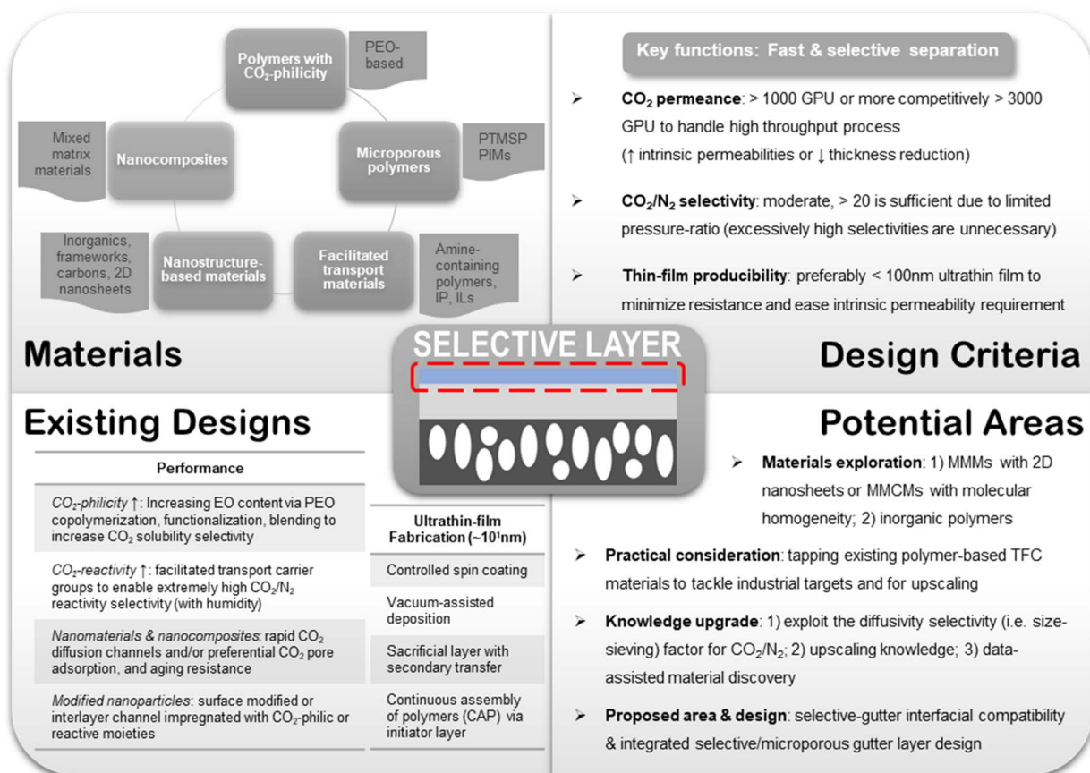
Fig. 9 Design summary for the selective layer.
