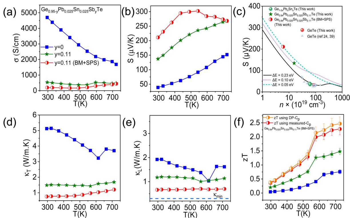
Fig. 4 Temperature dependent (a) electrical conductivity ( \sigma ), (b) Seebeck coefficient ( S ), (c) Pisarenko plot ( S vs. n ) at 300 K, (d) total thermal conductivity ( \kappa_T ), (e) lattice thermal conductivity ( \kappa_L ) and the (f) thermoelectric figure of merit ( zT ) of ingot and (BM + SPS) processed \text{Ge}_{0.84}\text{Pb}_{0.025}\text{Sn}_{0.025}\text{Sb}_{0.11}\text{Te} samples using measured C_p and Dulong–Petit (DP) C_p .
