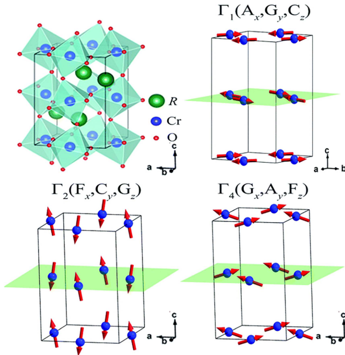
Fig. 2 The crystal and the spin structures of RECrO 3 .
