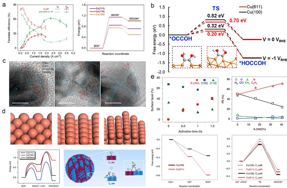
Fig. 8 (a) Different C_1 (short dashed) and C_{2+} (solid) product distributions of the hollow copper fiber (Cu HF, red) and activated Cu HF (green) as a function of current density (left). Activation energy barrier of OCCO^* and OCCOH^* from CO^* (right). Reproduced from ref. 167. Copyright 2022 Royal Society of Chemistry. (b) Reaction energy barriers for the formation of *HOCCOH from *OCCOH in synergy with Cu(611) and Cu(100) at 0 V_{RHE} and -1 V_{RHE} . The insets show the geometry of the system. Orange: Cu, red: O, grey: C, white: H. Reproduced from ref. 171. Copyright 2020 Proceedings of the National Academy of Sciences. (c) HR-TEM images of the crystal facets of HF-Cu, MF-Cu and LF-Cu catalysts; the blue dashed line circles Cu(100), the red dashed line circles Cu(111) facets and the yellow dashed line highlights the interface between the (100) and (111) facets. HR-TEM scale bar, 10 nm. (d) Geometrical schematics representing the Cu(111) and Cu(100) interfaces between Cu(111) and Cu(100) respectively (above). The reaction energy barriers for dimerization and trimerization reactions at the Cu(111) and Cu(100), and the interfaces between Cu(111) and Cu(100). Schematic diagram of a catalyst with highly mixed nanofragments of Cu(200) and Cu(111) facets on which C_1 and C_2 sites are very close together to facilitate C_1 - C_2 coupling and coupling into C_3 products (below). Reproduced from ref. 70. Copyright 2019 Nature. (e) Linear correlation between the fraction of surface facet and activation time on A-CuNW surfaces. A-(hkl) ratios correlated with product FEs at approximately -0.99 to -1.00 V vs. RHE (above). Adsorption energies ( \Delta G_{ads} ) of CO^* and 2CO^* on Cu(100) and Cu(511). The reaction coordinate of C_1 and C_2 pathways on Cu(100) and Cu(511). CO+^* represents CO and the active site on the surface before the adsorption of CO; CO^* represents the active site where CO was adsorbed. Reproduced from ref. 173. Copyright 2020 Nature.
