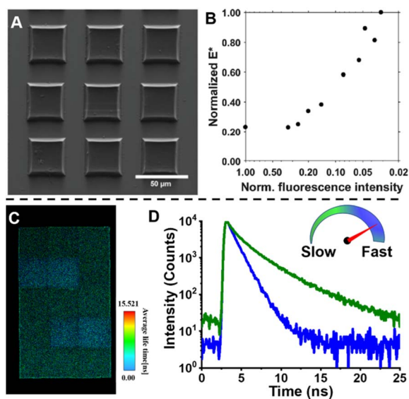
Fig. 19 (A) SEM image of microstructures containing only anthracene dimers as monomers. Reproduced from ref. 482 with permission from Wiley, copyright 2019. (B) Normalised complex modulus ( E^* ) determined by NanoDMA versus normalised fluorescence intensity of the structures shown in (A) determined by CLSM. Reproduced from ref. 482 with permission from Wiley, copyright 2019. (C) FLIM image of a microstructure made from two different photoresists, containing BODIPY-C12. Reproduced from ref. 490 with permission from The Royal Society of Chemistry, copyright 2022. (D) Fluorescence decay curves of BODIPY-C12 in the same microstructure as (C) showing BODIPY-C12 in different viscosity environments. Reproduced from ref. 490 with permission from The Royal Society of Chemistry, copyright 2022.
