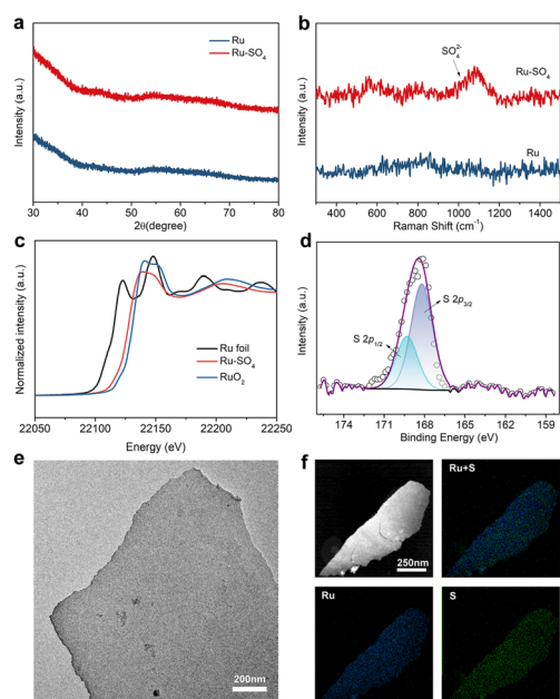
Fig. 1 (a) X-ray diffraction patterns of Ru and Ru-SO 4 . (b) Raman spectra of Ru and Ru-SO 4 . (c) Ru K-edge XANES of Ru foil, Ru-SO 4 and RuO 2 . (d) XPS spectra of S 2p for Ru-SO 4 . (e) Typical TEM image and (f) EDX mapping images for Ru-SO 4 .
