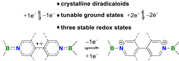
Fig. 1 Resonance forms and redox states of (a) Chichibabin's hydrocarbon and (b) viologens. (c) This work.
